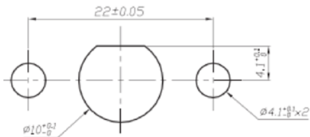
PANEL CUTOUT
